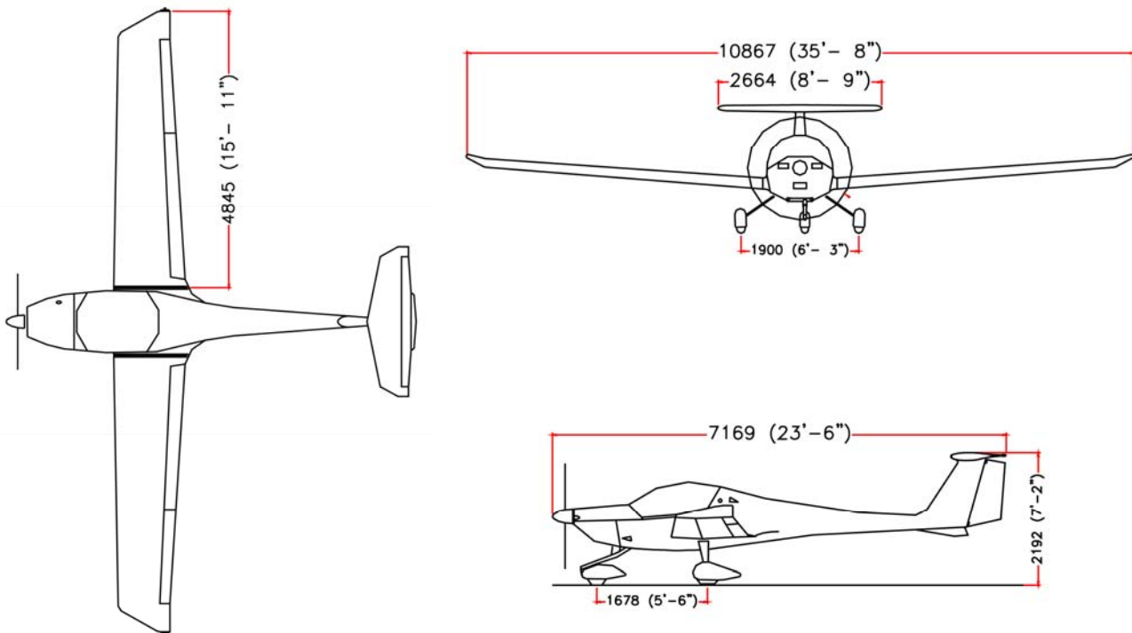
Three-View Drawing of DA20-C1 Aircraft
